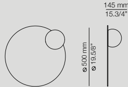
CIR_3702 LED 10W (2700K) Typ* 870 lumens Dimmable triac *Optional dimming available
